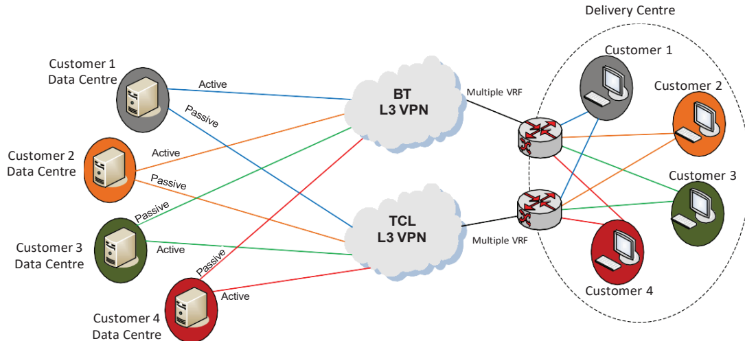
Figure: Multiple VRFs per customer
