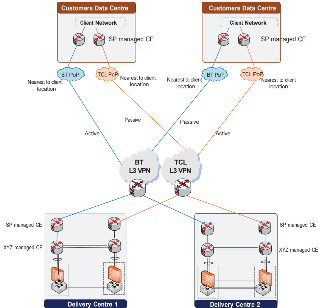
Figure: Client Connectivity
