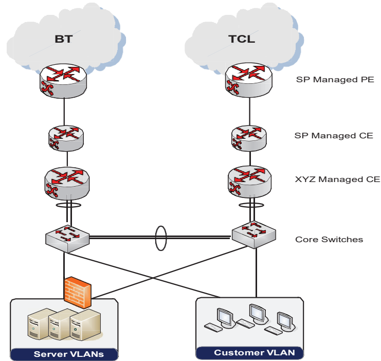
Figure: Client Connectivity
